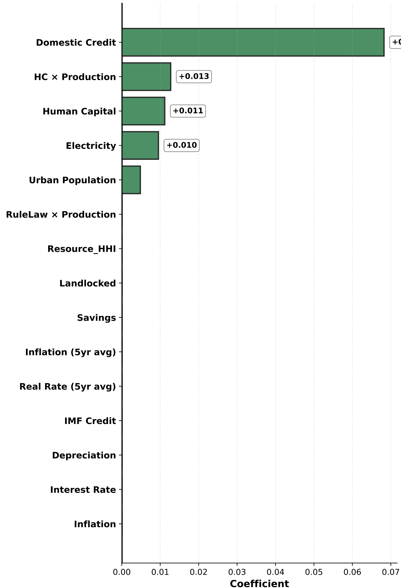
LASSO Train R 2 =0.769 Test R 2 =0.857 | 6 features
